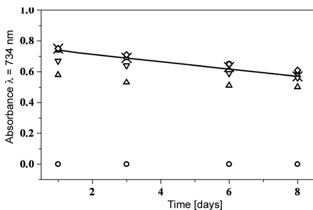
Fig. 3. Time effect on the suppression of the absorbance (at 734 nm) of the ABTS •+ . Control ABTS •+ (x). Trolox: 10 \mu M (○), 1 \mu M (△), 0.5 \mu M (▽), 0.1 \mu M (□) [overlapped with (◇) and (x)] and 0.01 \mu M (◇).
