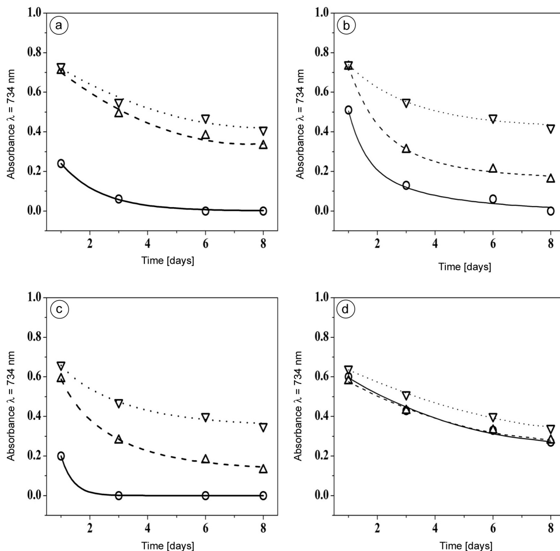
Fig. 4. Time effect on suppression of \text{ABTS}^{\bullet+} absorbance at 734 nm (averages of 2 measurements). (a) 1 3' II 8 biapigenine (amentoflavone), (b) 4'-methoxy 5,7-dihydroxyflavone 6-C- \beta -glucopyranoside (isocytiside), (c) 7-O- \beta -[2-O-feruloyl- \beta -glucuronopyranosyl (1 \rightarrow 2) glucuronopyranoside] (tricine), (d) all- trans \beta -carotene; concentrations 10 \mu\text{M} (—○—), 1 \mu\text{M} (--- \Delta ---) and 0.5 \mu\text{M} (··· \nabla ···).
