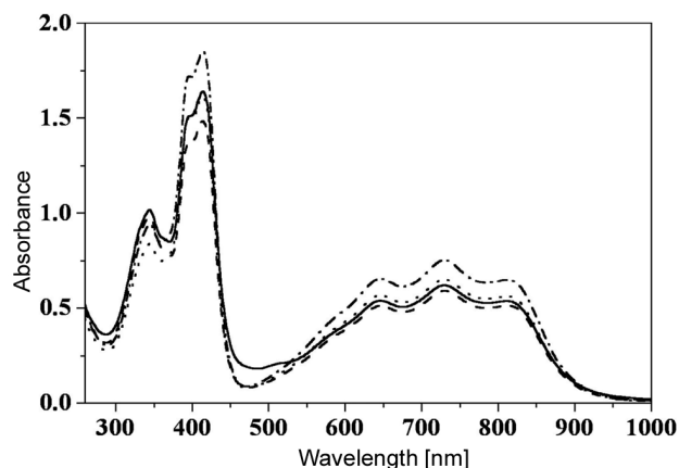
Fig. 6. Effect of 10 µM (—), 1 µM (---) and 0.5 µM (···) β-carotene concentrations on suppression of the ABTS + control signal (—·—).
