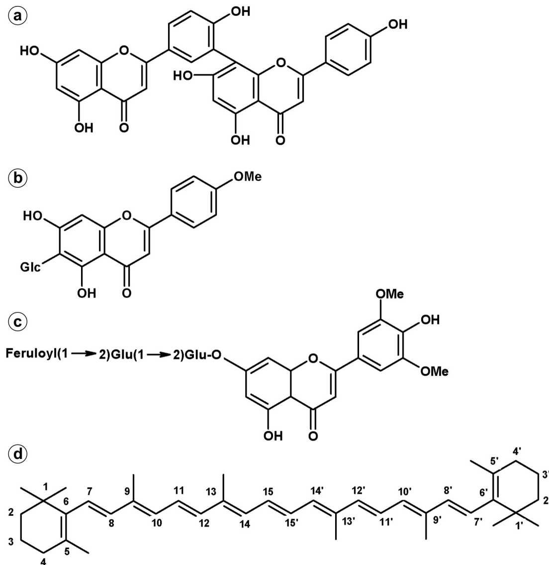
Fig. 2. Molecular structure of the applied flavonoids: (a) 1,3'-di-O-8-biapigenin (amentoflavone), (b) 4'-methoxy 5,7-dihydroxyflavone 6-C- \beta -glucopyranoside (isocytiside), (c) 7-O- \beta -[2-O-feruloyl- \beta -glucuronopyranosyl (1 \rightarrow 2) glucuronopyranoside] (tricine), (d) all- trans \beta -carotene.
