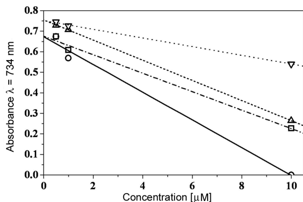
Fig. 5. Effect of flavonoid and trolox concentration on suppression of ABTS + absorbance at 734 nm. Trolox (O), I 3' II 8 biapigenine (amentoflavone) (△), 4'-methoxy 5,7-dihydroxyflavone 6-C-β-glucopyranoside (isocytiside) (▽), 7-O-β-[2-O-feruloyl-β-glucuronopyranosyl (1→2) glucuronopyranoside] (tricine) (□).
