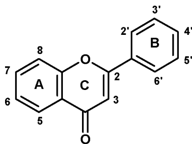
Fig. 1. Basic structure of flavonoid molecule.
